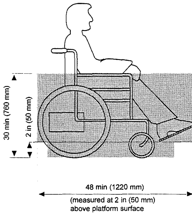
WHEELCHAIR OR MOBILITY AID ENVELOPE
