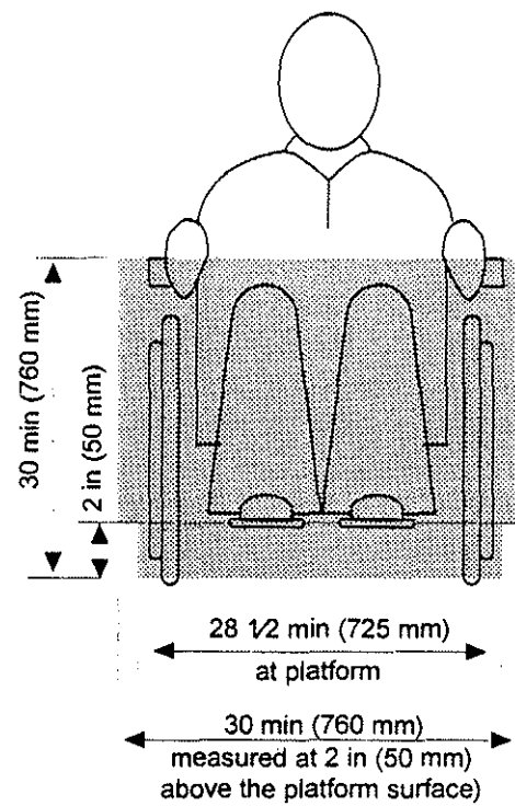
WHEELCHAIR OR MOBILITY AID ENVELOPE
